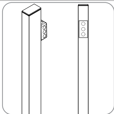
2"X4" J-BOX
