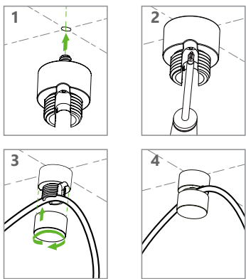
Hook (TDSH) Stand Alone installation sequence
