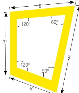
TOP VIEW - Corner Pattern
