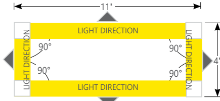
Ships with corner element assembled to luminaire(s)
