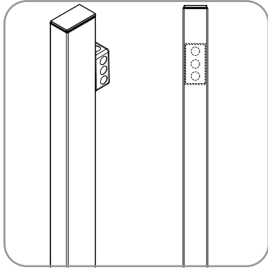
2"X4" J-BOX
