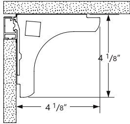
Section view - Ceiling-to-Wall Corner Mount
