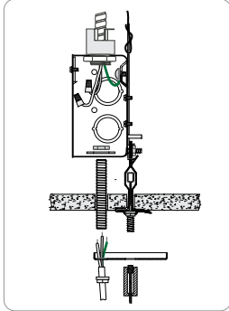
CT TILE CEILING-ON GRID
