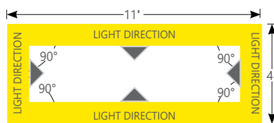
TOP VIEW - Rectangle Corner Pattern
